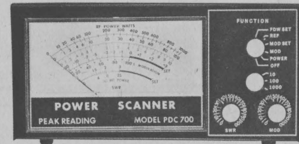
MODEL PDC 700
